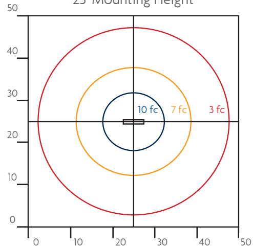
IES Type Distribution: V 25' Mounting Height
